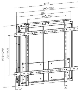
Dimensions (mm)
